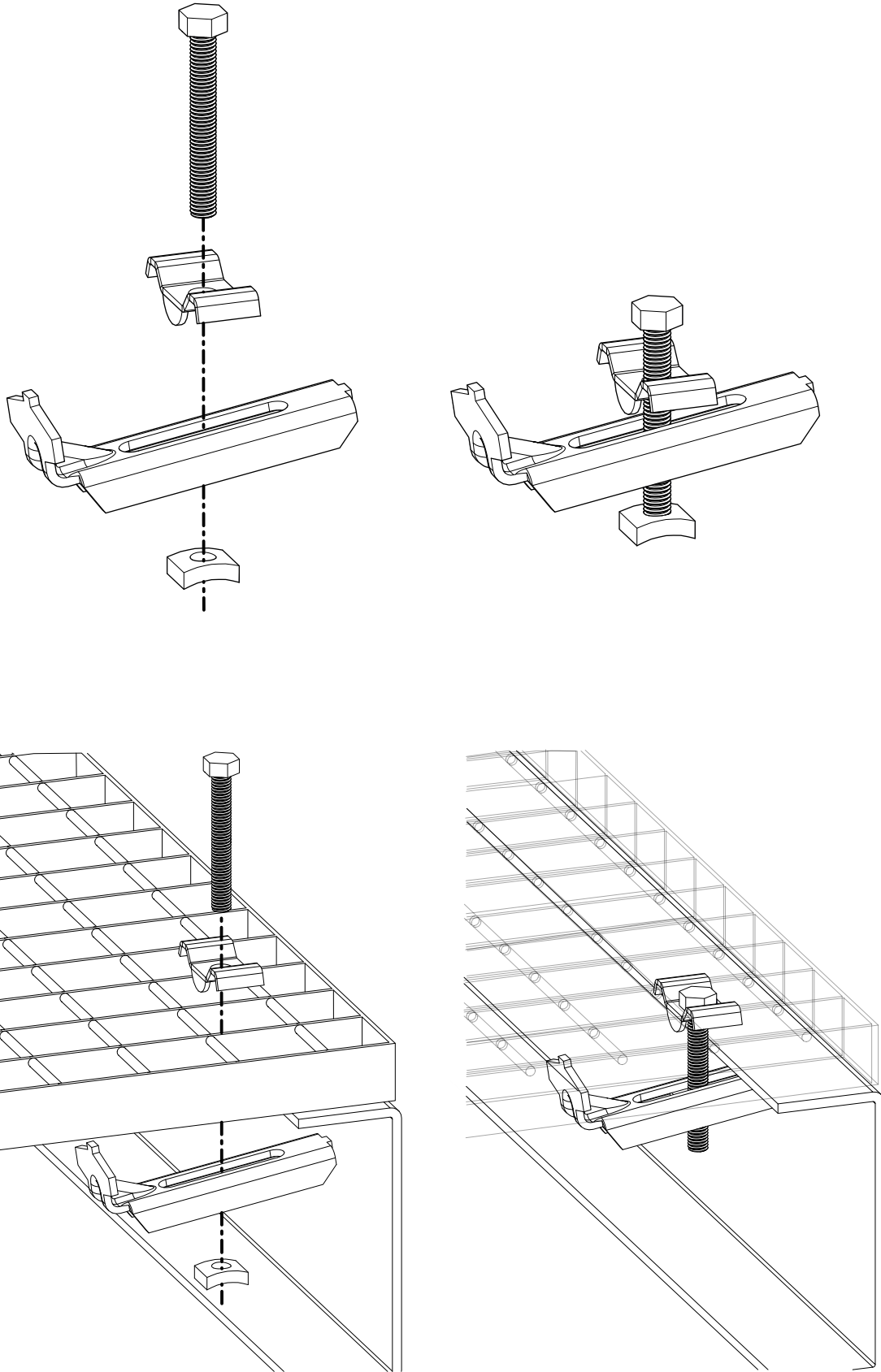
Assembly instruction - Complete fixing for grating Method shows grating Type A & U steel beam
