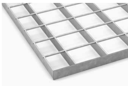
14 - Mesh Width 68 x 50 mm
